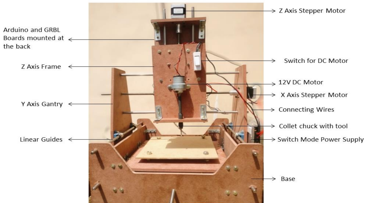
Figure 3: Fabricated Mini CNC Milling Machine
