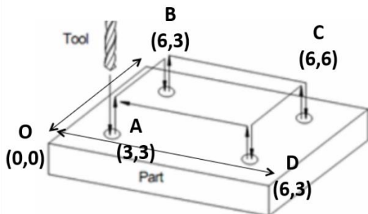
Figure 4: Coordinate Measuring Test for Checking Accuracy of Machine
